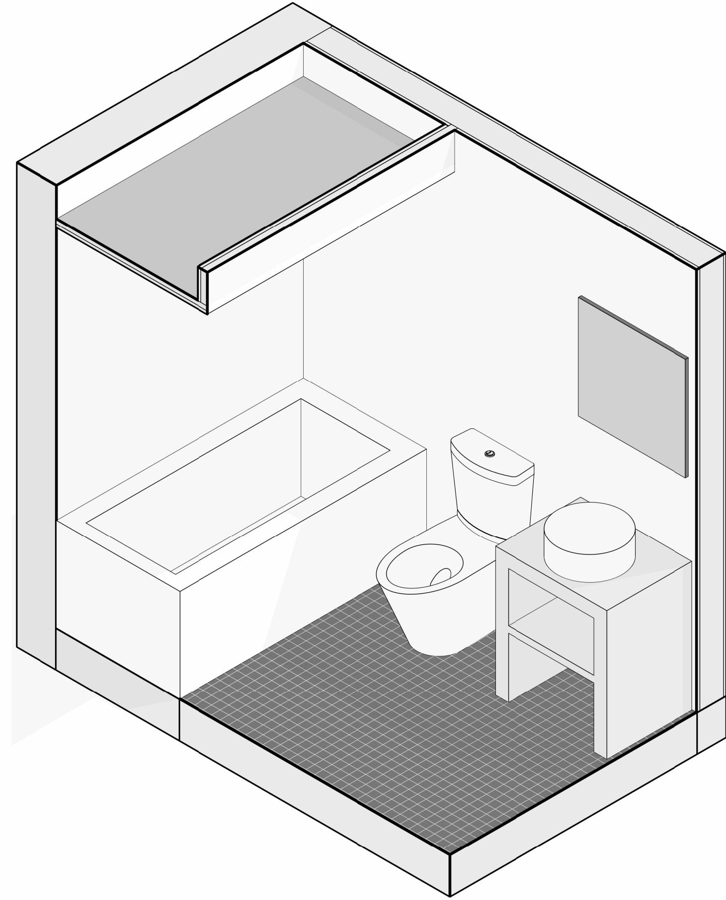
4 Bathroom Axon
