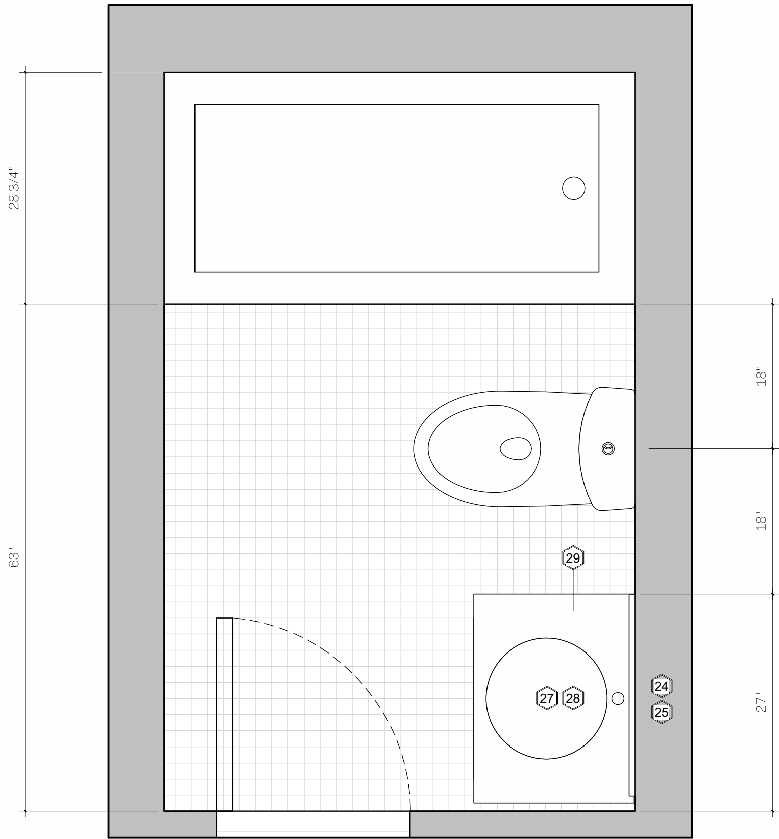
1 BATHROOM PLAN 1" = 1'-0"
