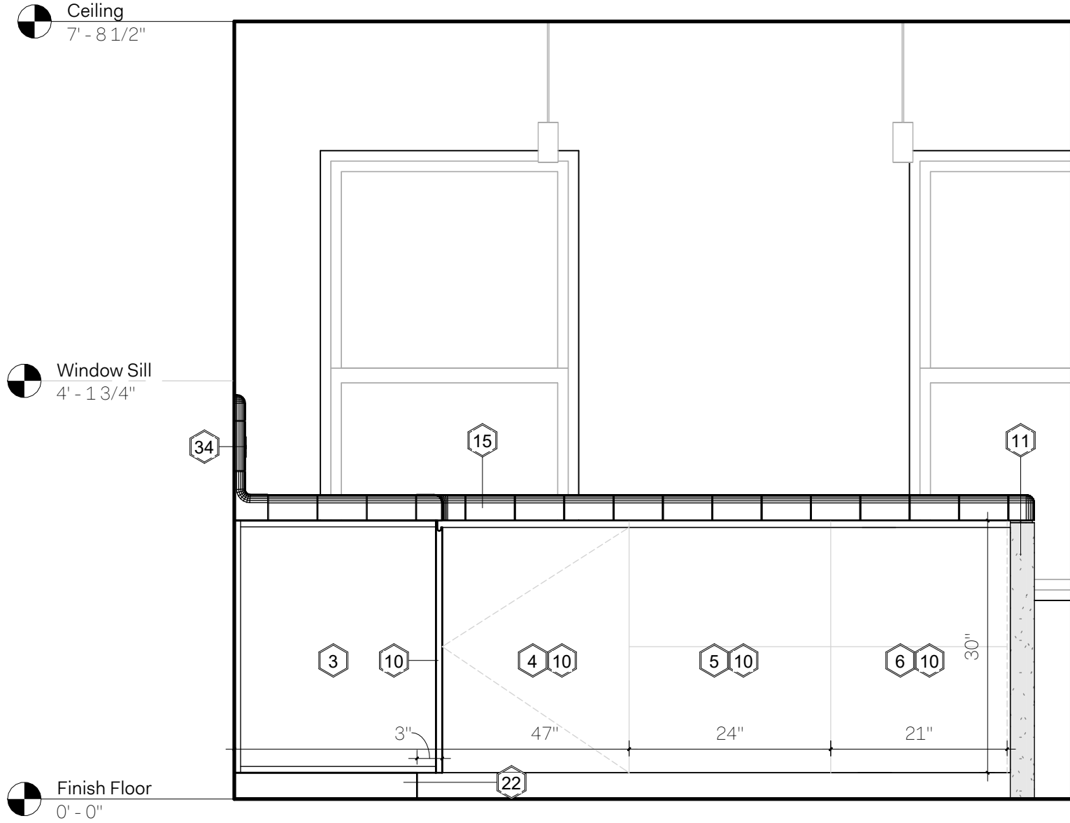
1 Kitchen Elevation East 3/4" = 1'-0"
