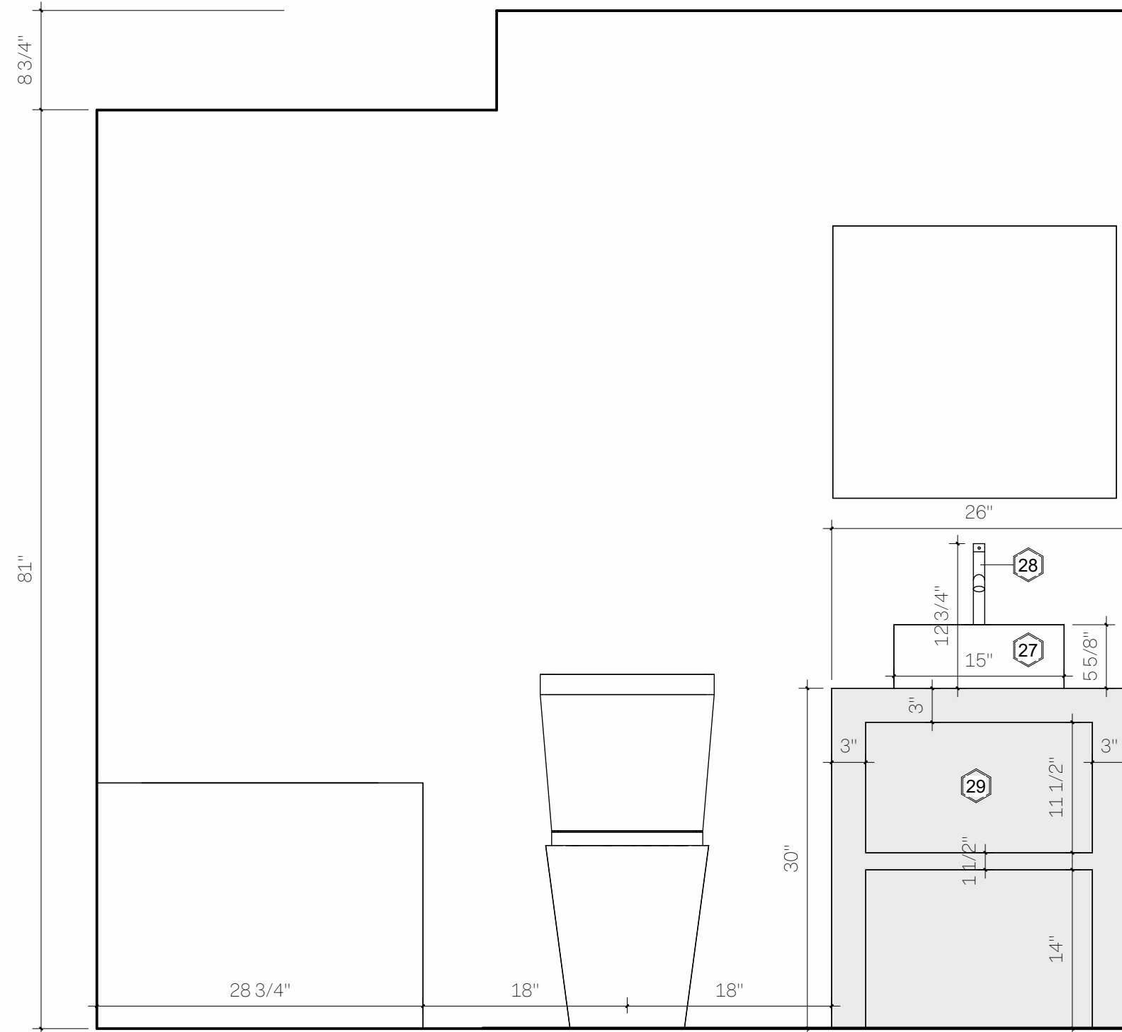
2 BATHROOM C 1" = 1'-0"
