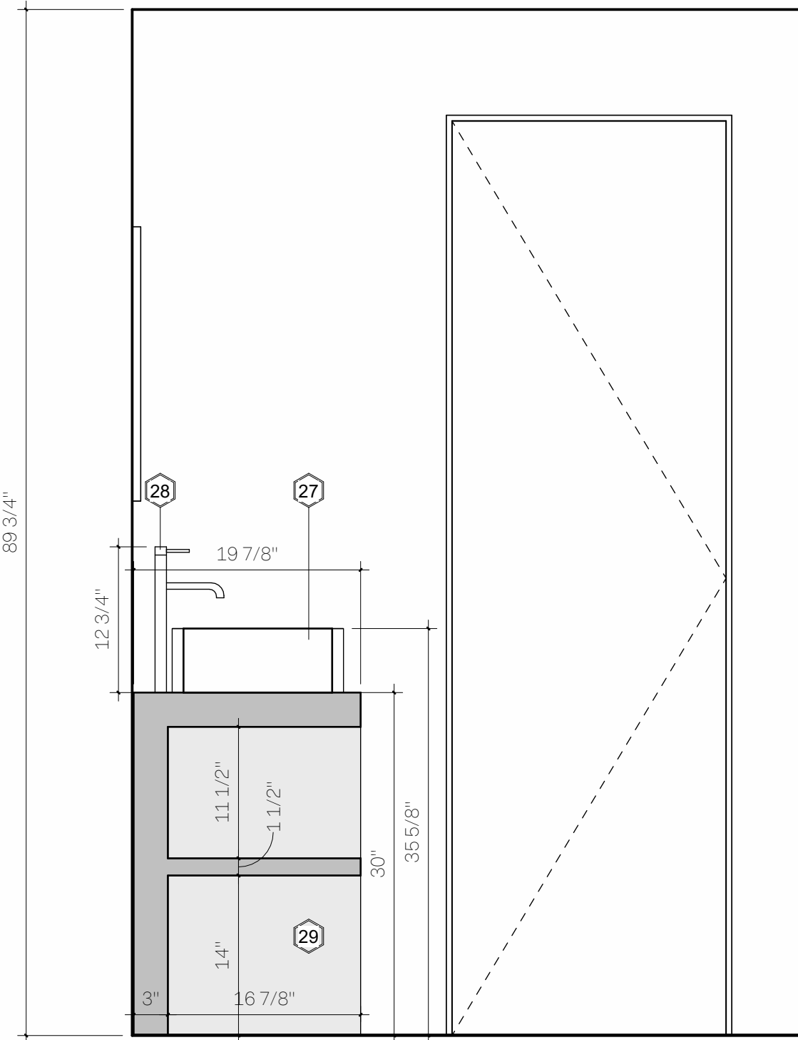
3 BATHROOM D 1" = 1'-0"
