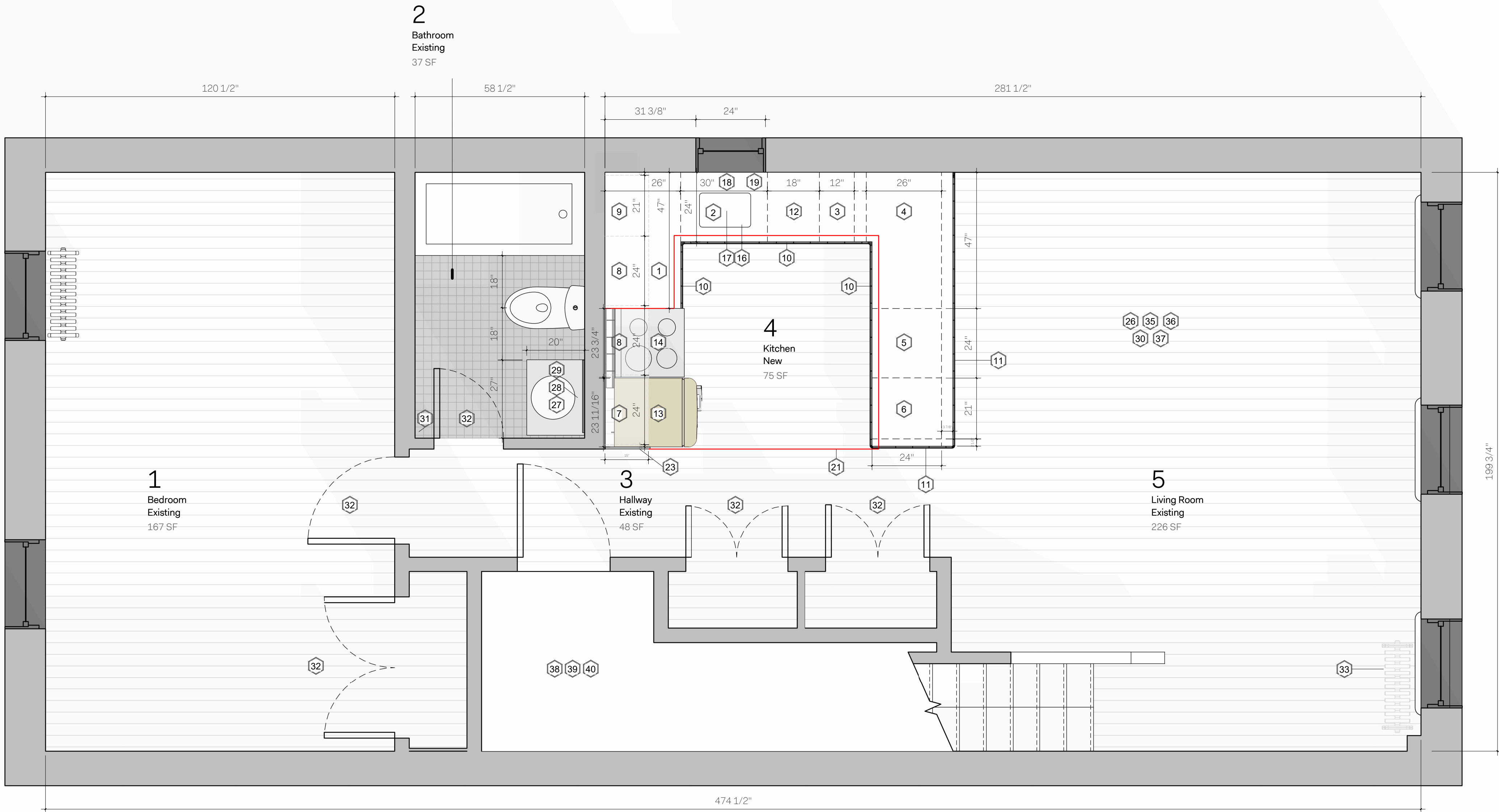
1 Construction Floor Plan 1/2" = 1'-0"
