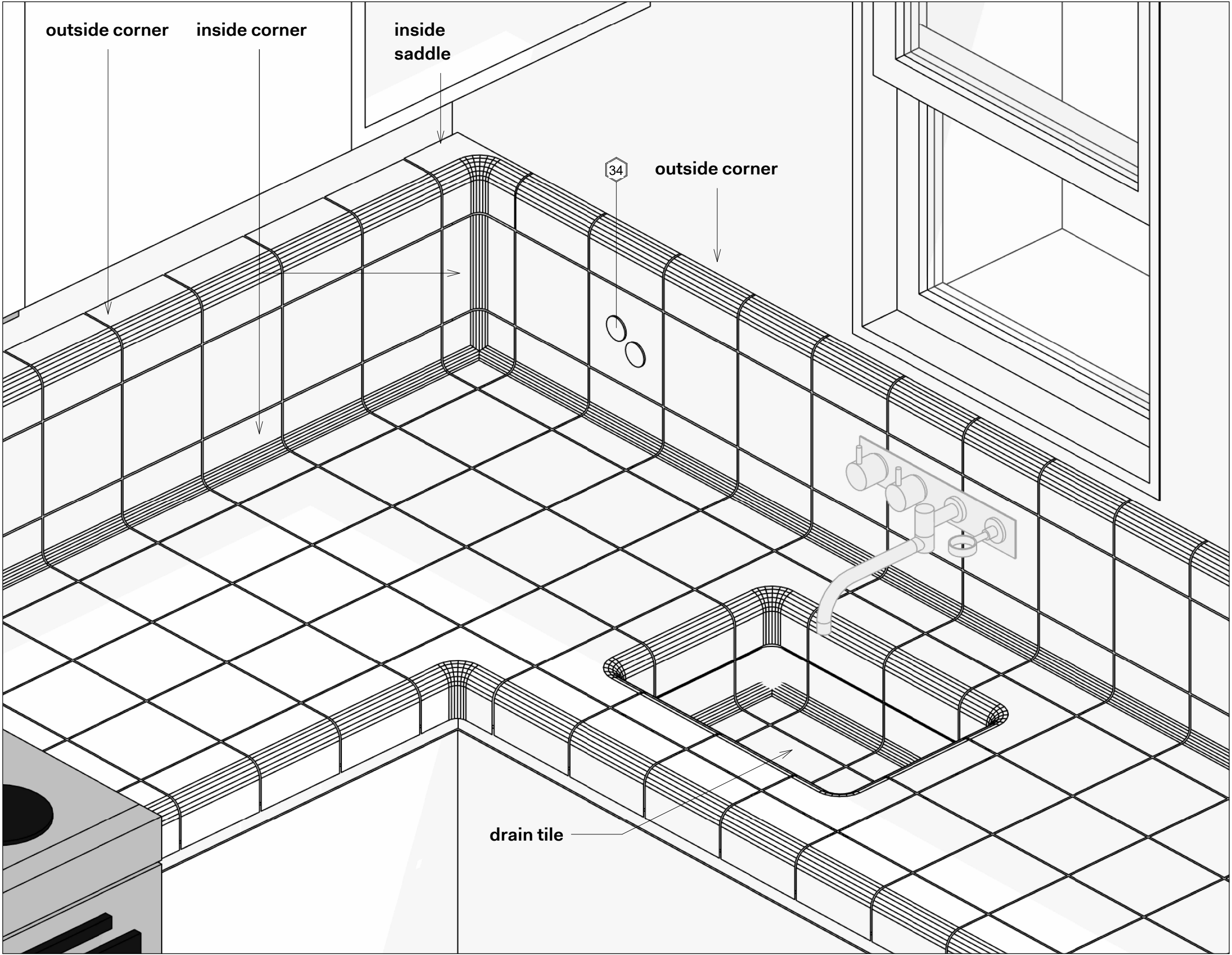
Tile Counter Corner Detail
