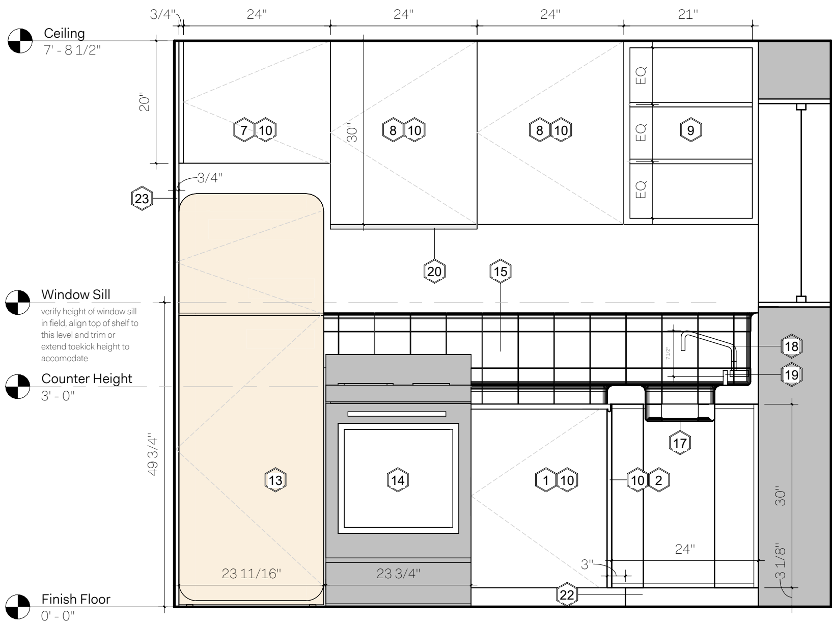
3 Kitchen Elevation West Option 1 3/4" = 1'-0"
