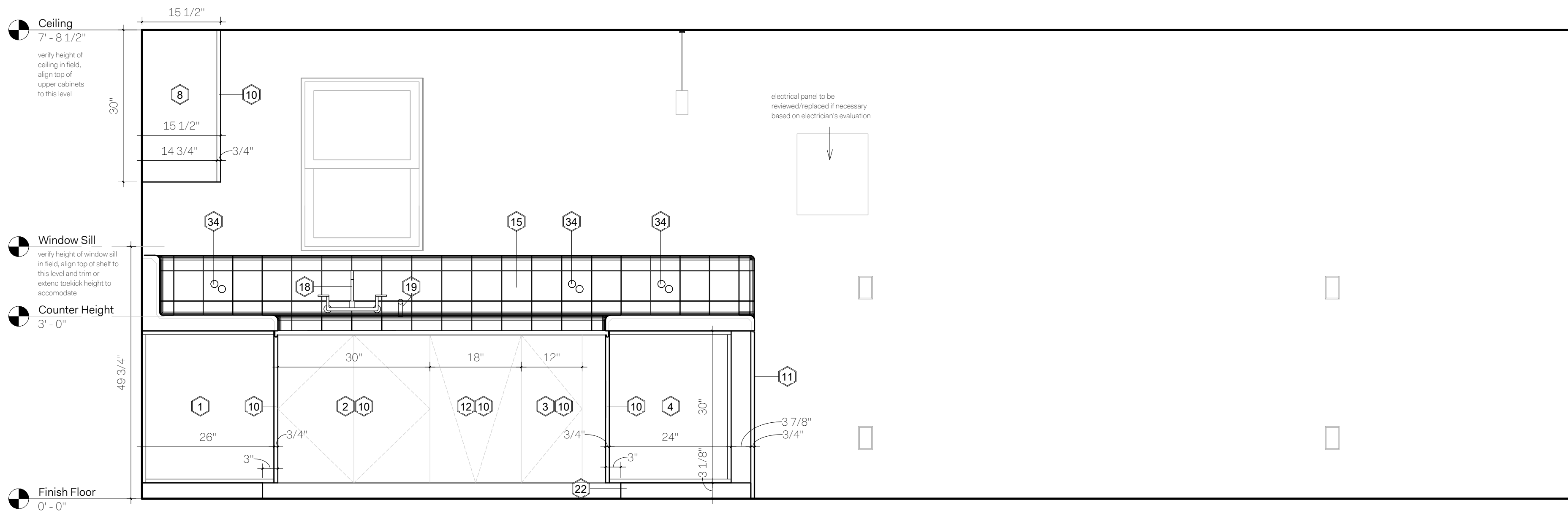
2 Kitchen & Living Elevation North 3/4" = 1'-0"
